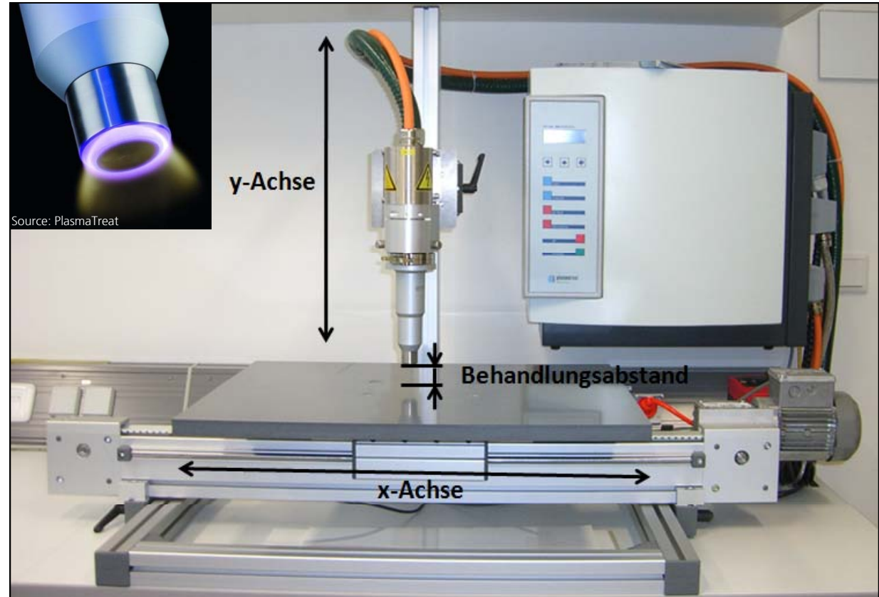
Plasma pretreatment system with linear table, plasma outlet at the rotary nozzle
